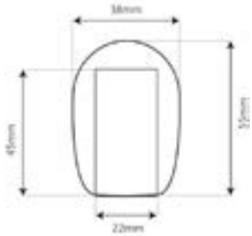
G122CC FOAM MICROPHONE WINDSHIELDS 22MM 3 PK Black foam windshield. Pack of 3.
