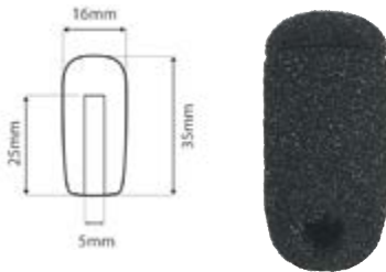
G122CJ FOAM MICROPHONE WINDSHIELD 5MM Black 5 mm foam windshield.
