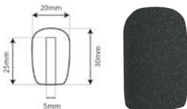
G122CF FOAM MICROPHONE WINDSHIELD 5MM Black 5mm foam windshield.
