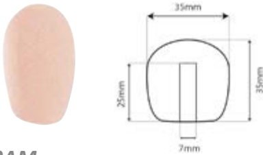
A090AM FOAM MICROPHONE WINDSHIELD FLESH COLOURED Windshield to fit the A090AL
