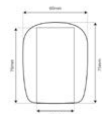
G132DA FOAM MICROPHONE WINDSHIELD 45MM PK OF 5
