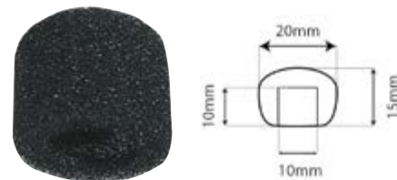
G122CK FOAM MICROPHONE WINDSHIELD 10MM Black 10 mm foam windshield.
