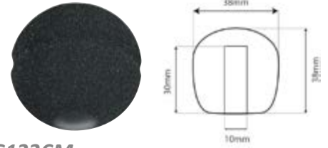
G122CM FOAM MICROPHONE WINDSHIELD 10MM Black 10 mm foam windshield.
