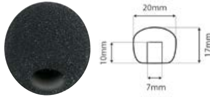
G122CG FOAM MICROPHONE WINDSHIELD 7MM Black 7 mm foam windshield.
