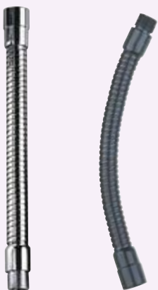
HEAVY DUTY GOOSENECKS WITH STANDARD FITTING Goosenecks in chrome OR black finish with standard male and female 5/8" x 27tpi threads.
